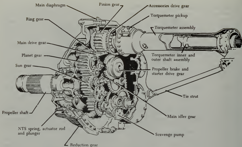
FIGURE 7-33. Reduction gear and torque meter assemblies.
